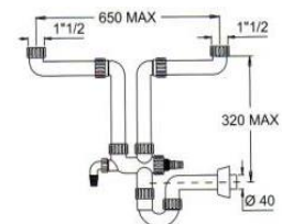
Sifone Industriale 2 Vie 11/2" S12V11\2
