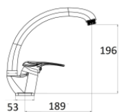
Mix Debora Lavello Monof. Canna Alta Pes. Gran. Beige MLMLDE85
