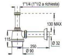
Sifone 1 Via 11/4" S /Piletta S1V11\4
